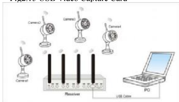
Fig2.15 USB Video Capture Card
